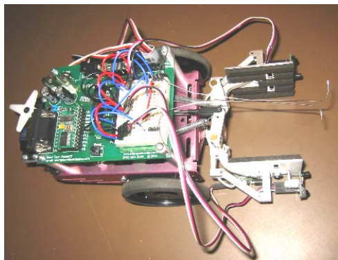
Fig. 9 - Termite (Boe-Bot with gripper)
