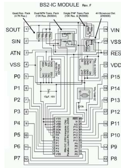
Fig. 8 - BS2-IC schematic
