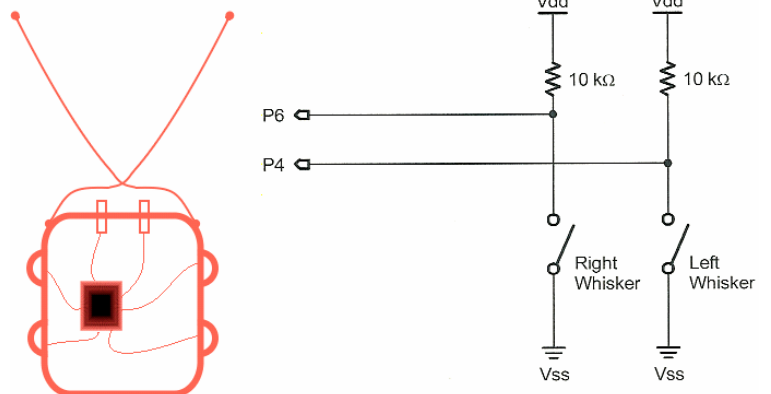
Whiskers Schematic.
