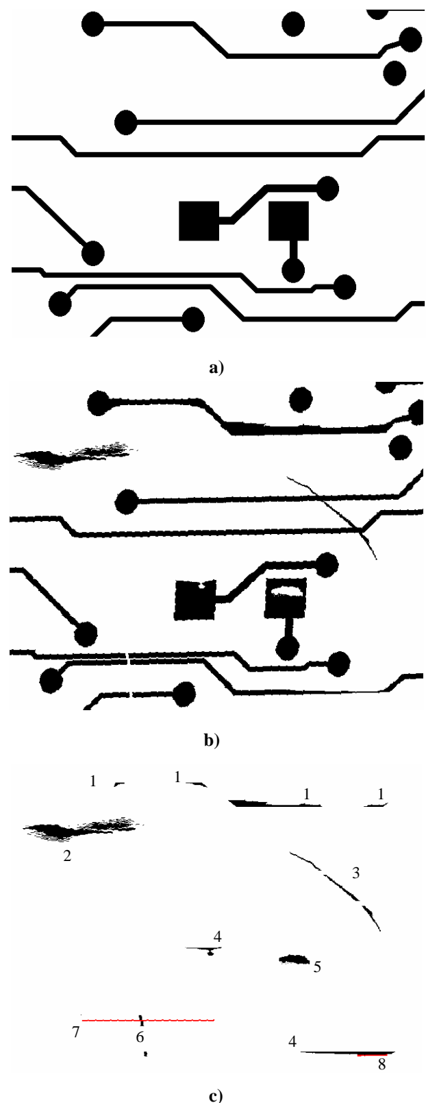
Fig. 2 - The reference PCB layout image. (a): processing image. (b): found defects. (c): 1) spur, 2) spurious copper, 3) short, 4) mousebit, 5) pin hole, 6) breakout, 7) distance between conductors is less than project rules, 8) the width of a conductor is less than project rules.
