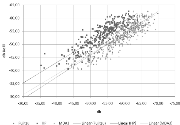
Fig. 9 - Scatter-plot of correlated RSSI-values
