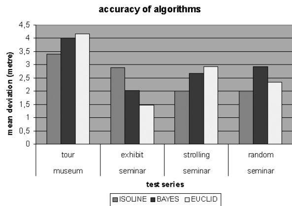
Fig. 10 - Comparing the accuracies of three algorithms
