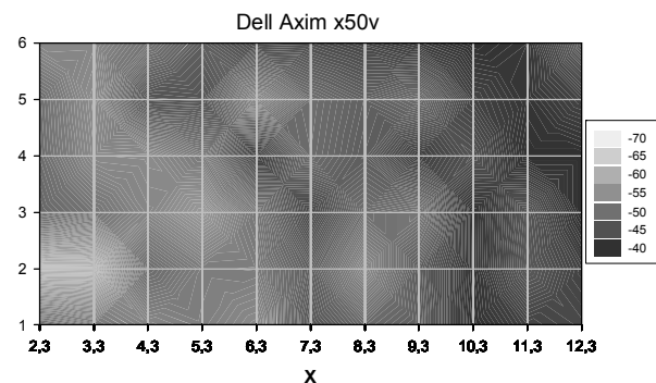
Fig. 7 - Radiomap recorded by a Dell PDA (testbed 1, AP1, orientation 0 degree)
