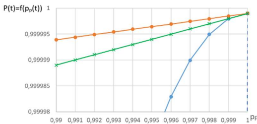
Figure 14. Graphs of the dependence (a, b) of the PF of RCPU structures St1, St2, St3, St4 on the PF of the SW of the first (main) channel if p_a(t) = 0,99999 ; p_{a1}(t) = 0,9995 ; p_{p1}(t) = 0,9995 ; P_{CDT}(t) = 0,999999 .
