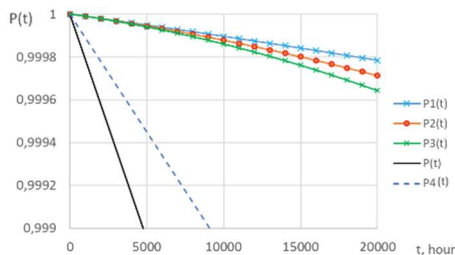
Figure 7. Graphical dependencies of PF structures RCPU St0, St1, St2, St3, St4 on time until the failure \lambda_a = 10^{-7} 1/h, \lambda_p=10^{-7} 1/h, \lambda_{a1}=10^{-6} 1/h, \lambda_{p1} = 10^{-6} 1/h, \lambda_{CDT}=10^{-8} 1/h.
